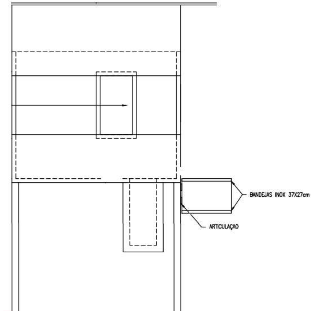
Vista frontal
